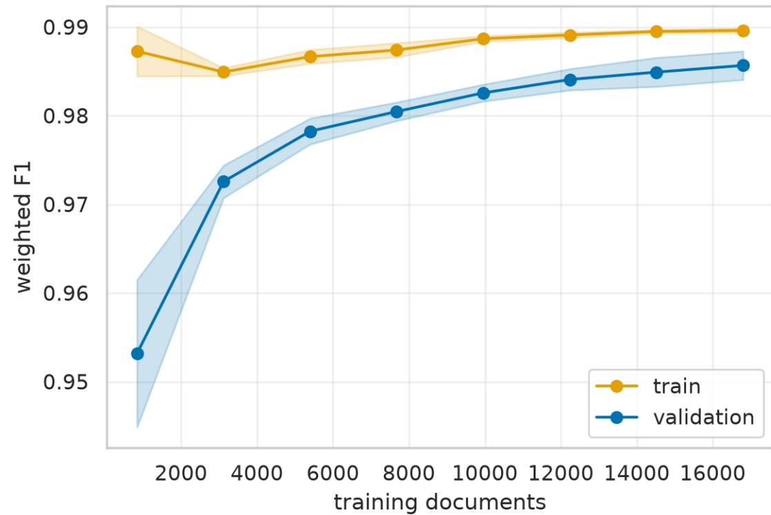
DAIGT V2: learning curve (LogReg, TF-IDF)
