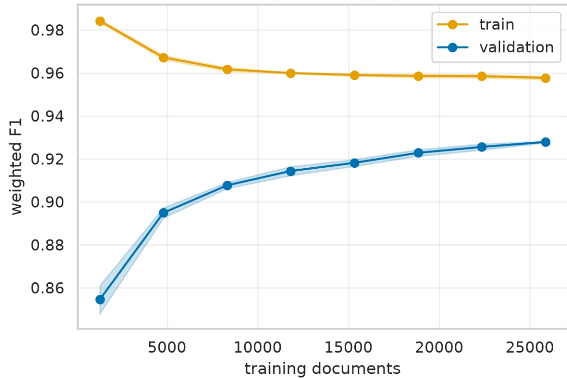
HC3: learning curve (LogReg, TF-IDF)
